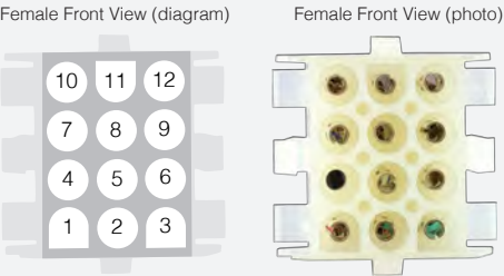
Plug/Wire Bundle Diagram 1
